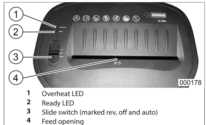
Fig. 1 Controls intimus 21 CP4
