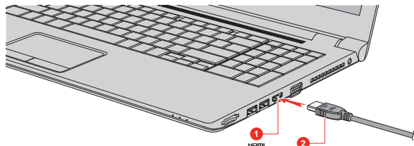
Figure 4-18 Connecting the HDMI™ out port
