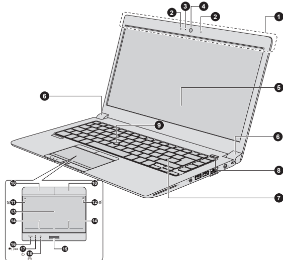
Figure 3-12 The front of the computer with the display panel open (Z40-C)
