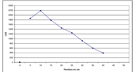
Lux curve
